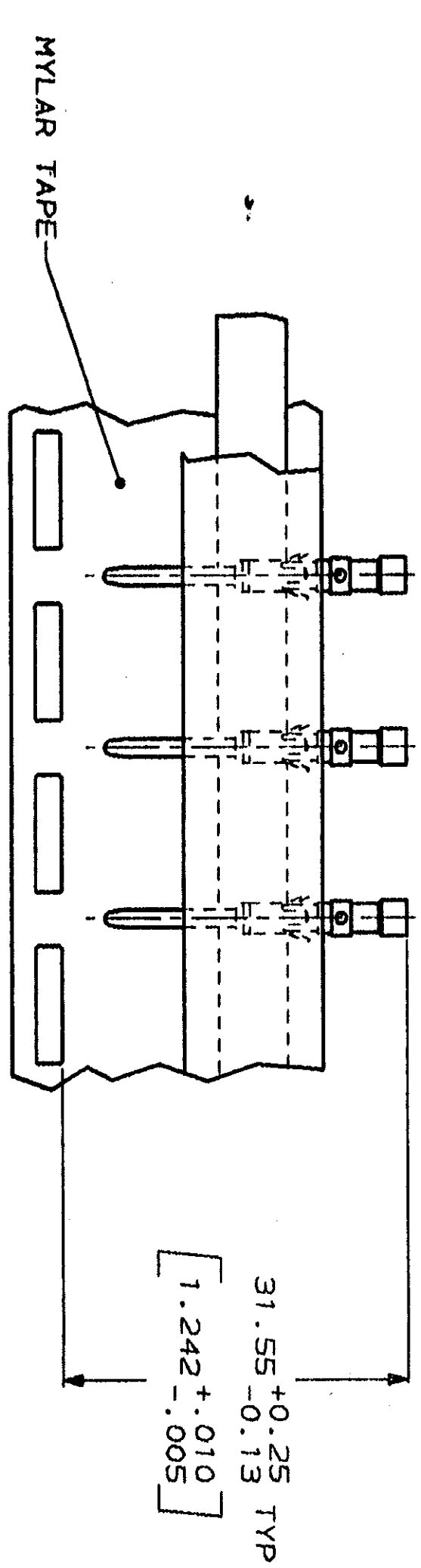
TAPE MTG DETAIL SCALE 2:1
